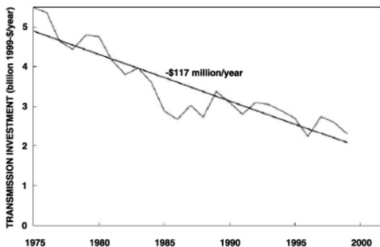
Fig. 3. Annual transmission investments from 1975 through 1999.
