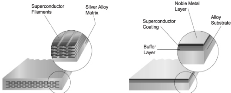
Multi-Filamentary Composite (AMSC commercial, in production)
